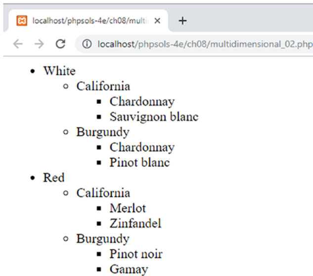
Figure 8-7. ListBuilder extends RecursiveIteratorIterator to automate building nested lists from a multidimensional associative array
